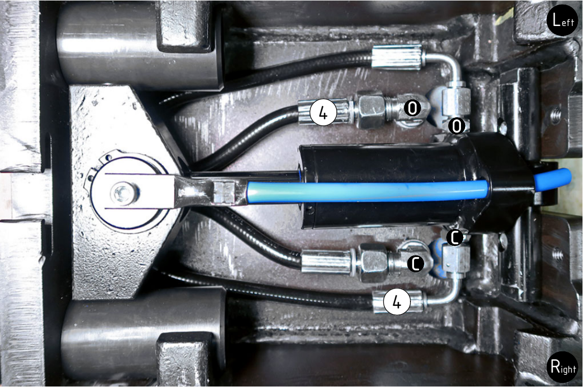
Hoses as far away from moving parts as possible!
