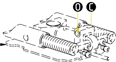
Exploded view Std. Hitch components
