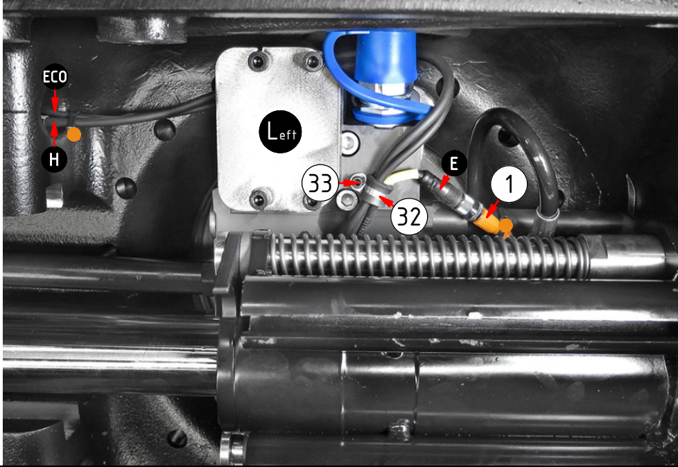
Sensor Cables
