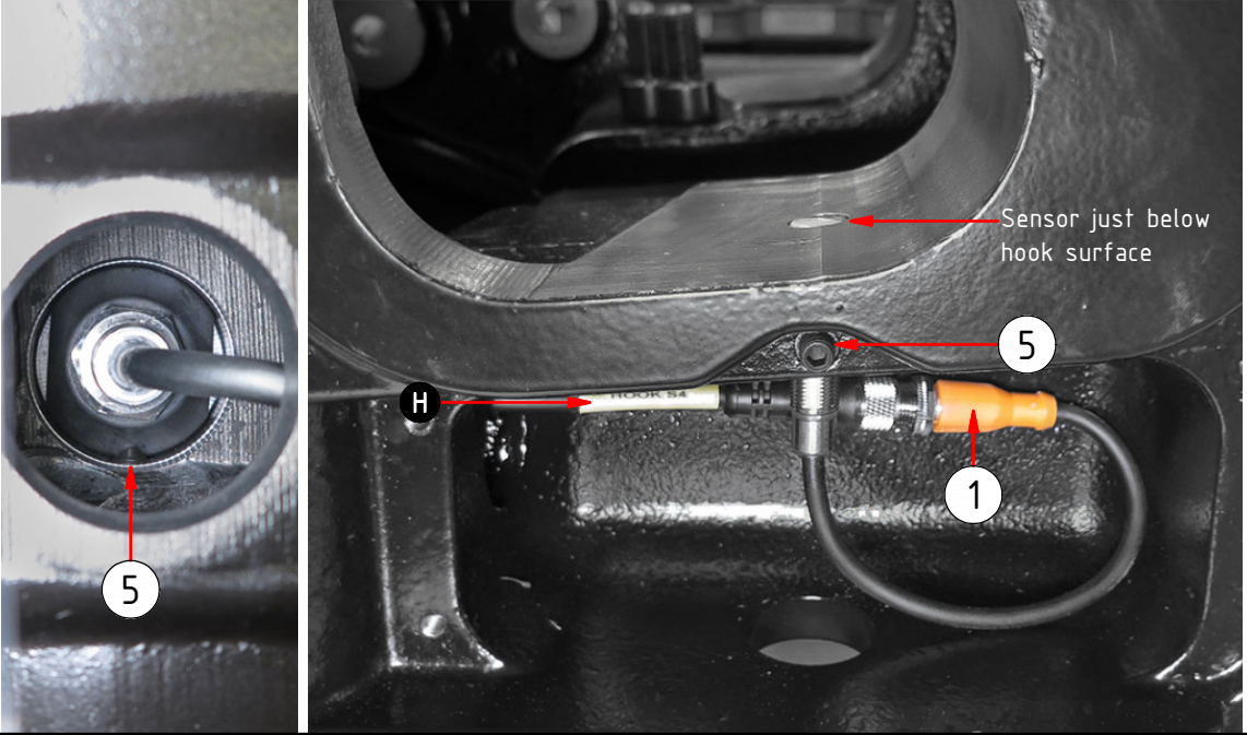
Sensor Hook
