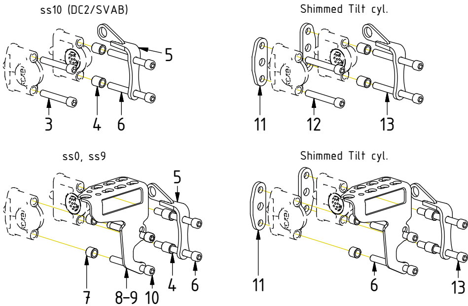
Feed 3/4" (option)
