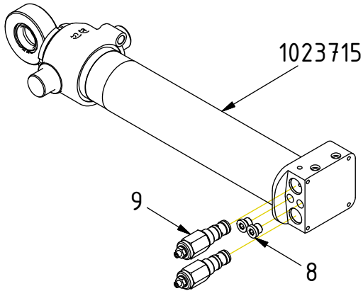
Tilt cylinder incl. Overcentre
