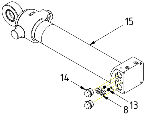
Tilt cylinder incl. Plugs
