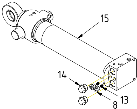
Tilt cylinder incl. Plugs
