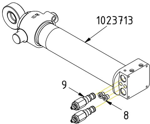
Tilt cylinder incl. Overcentre
