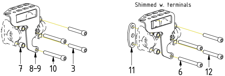
Feed 1/2" (option)
