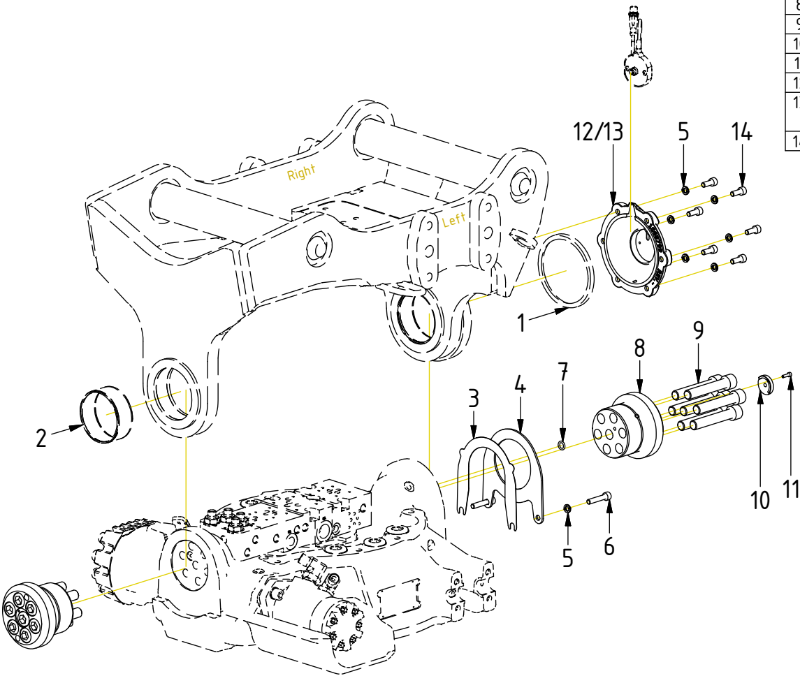
Exploded view ePS2 Sensors
