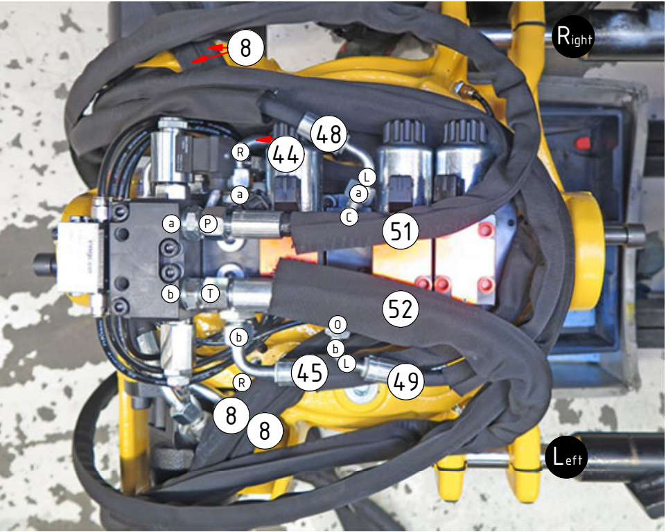
Rotation hoses crossed behind valve block, all hoses go to the left.
