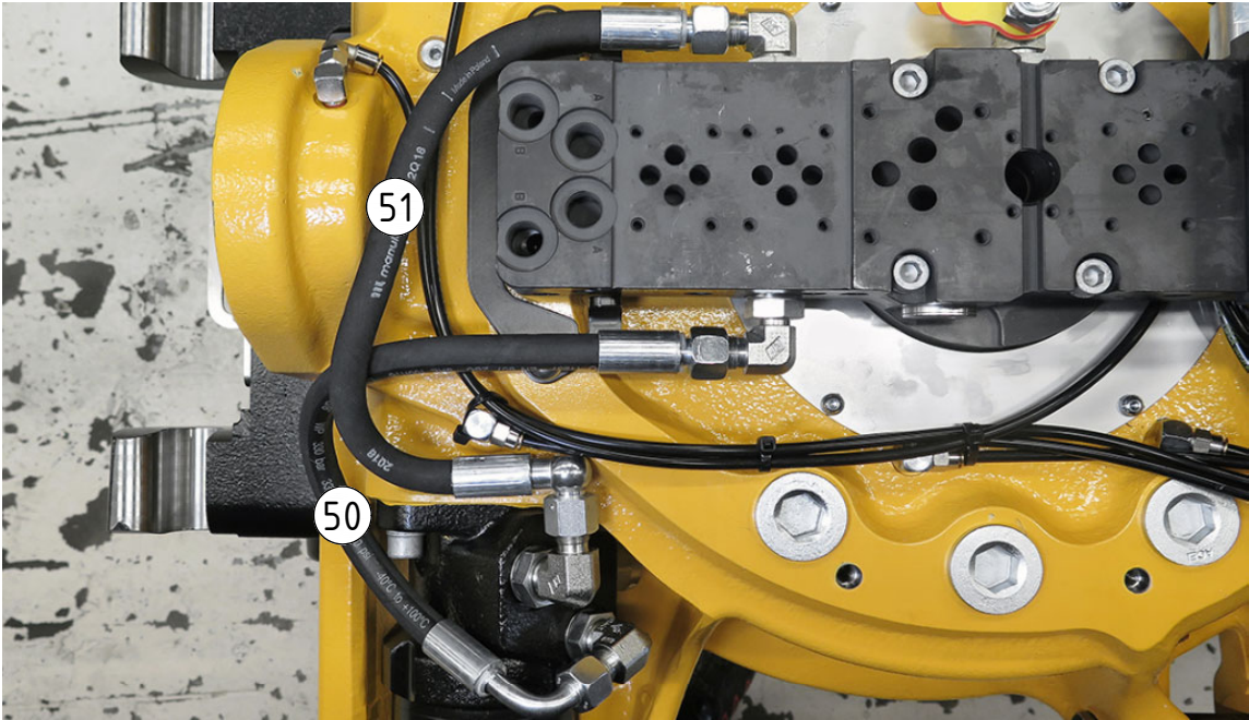
Motor hoses
