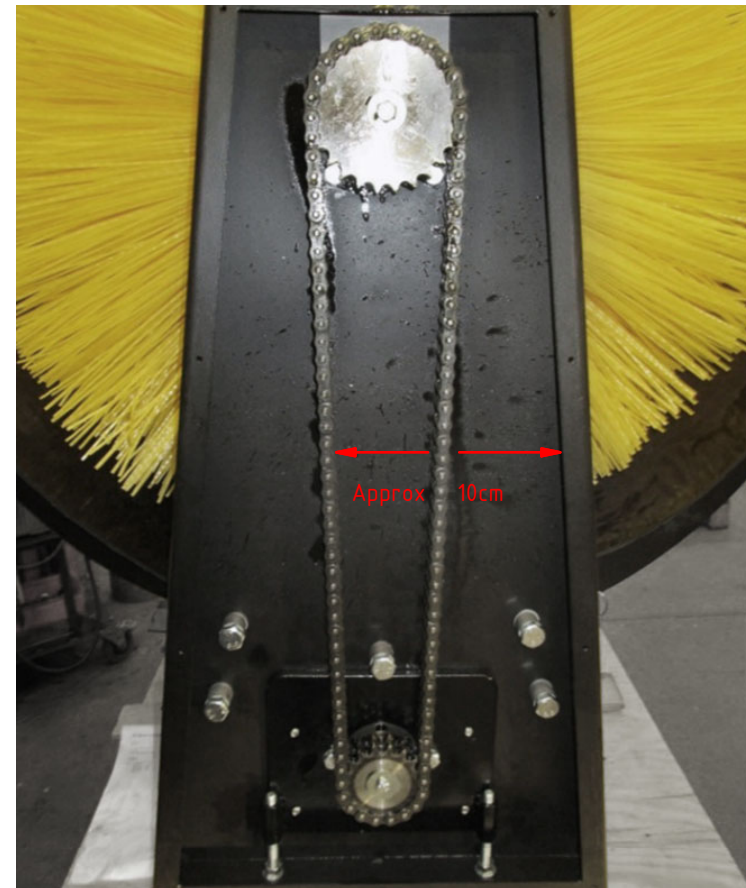
NB! The 2 furthest segments on each side mounts in same direction
