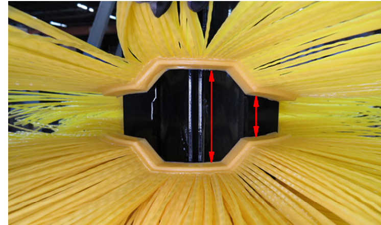
NB! The 2 furthest segments on each side mounts in same direction
