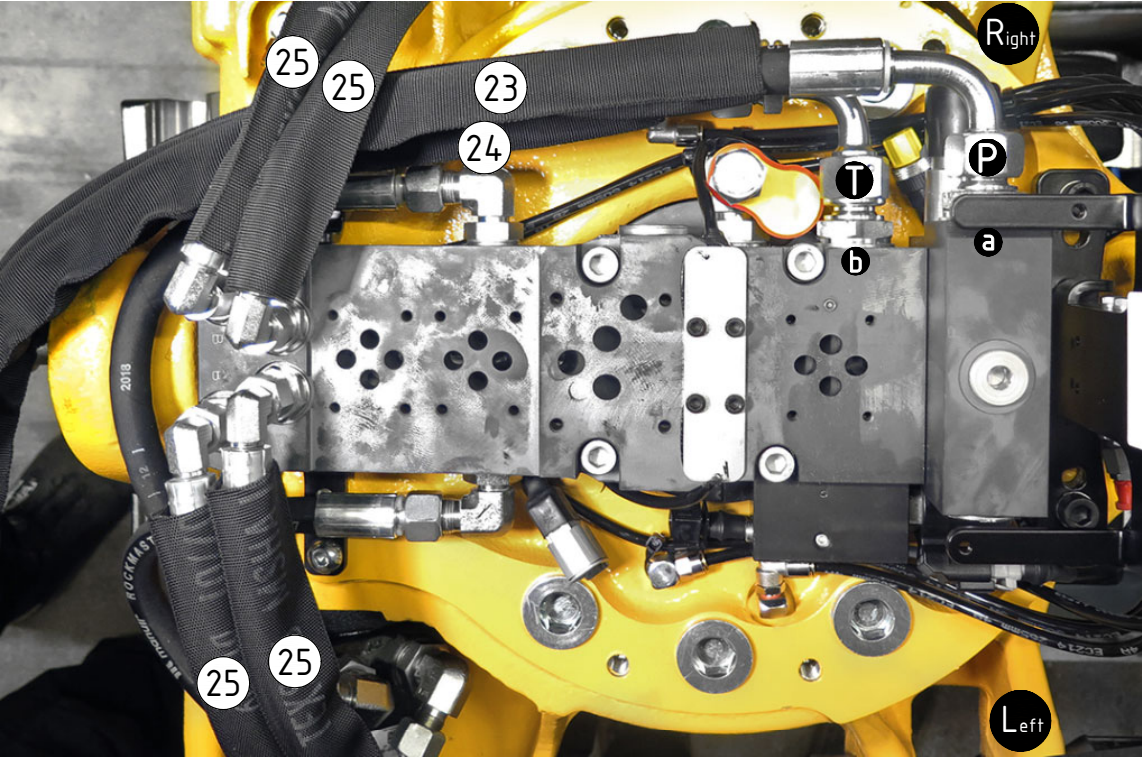
Hoses EC-Oil
