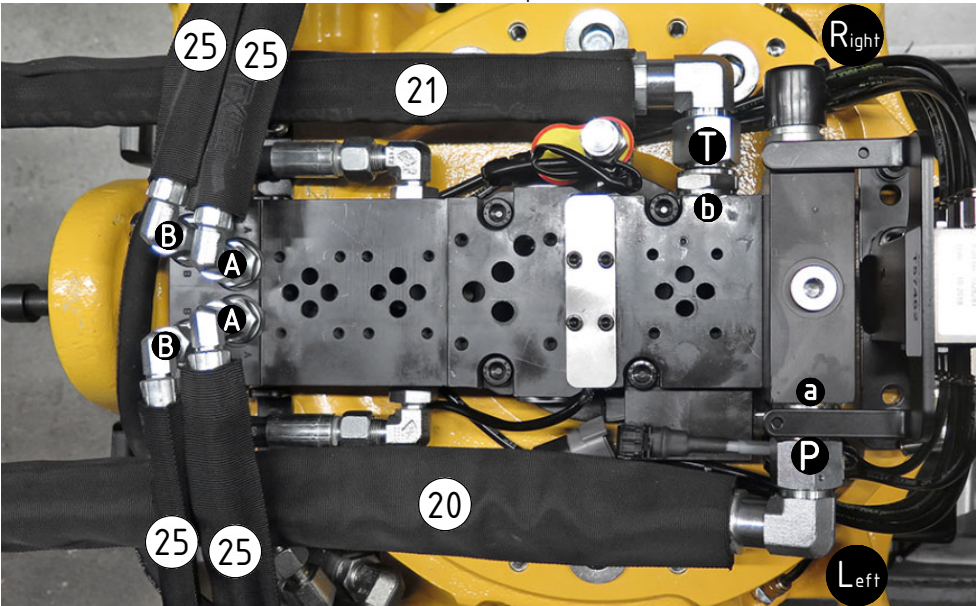
Feed 3/4" (option)
