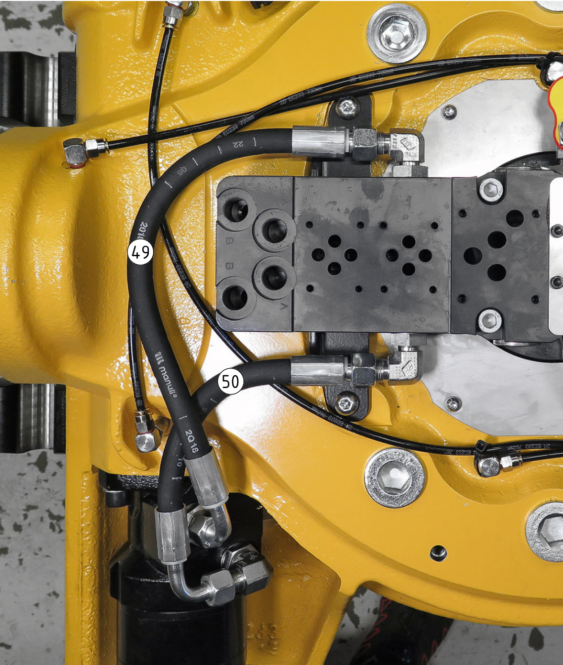
Motor hoses
