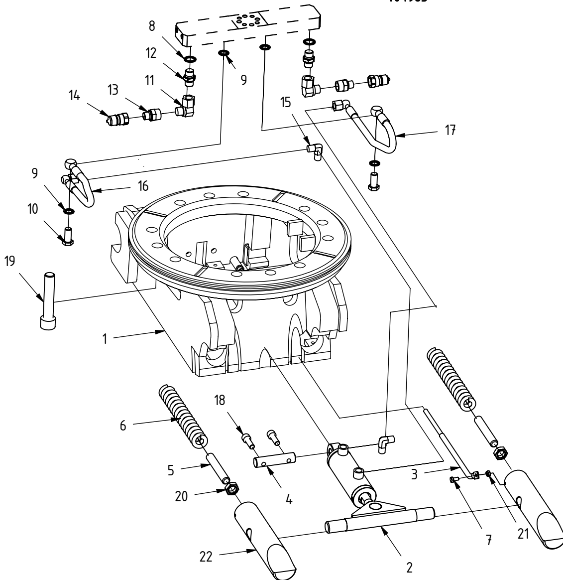
Complete Component Drawing for Lockcylinder 400849K (pos. 2): 404965
