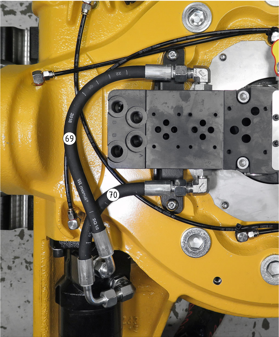
Motor hoses
